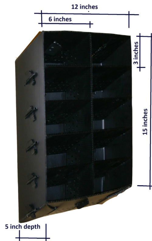
FIGURE 2. Dimensions of typical chloroplast greenwall planter box.
