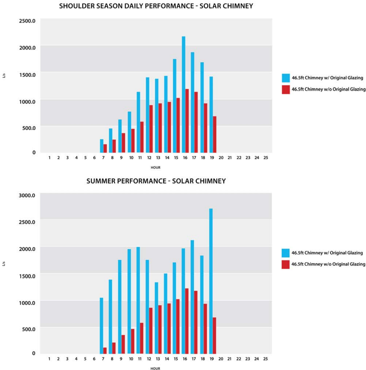
FIGURE 6. Solar chimney performance.
