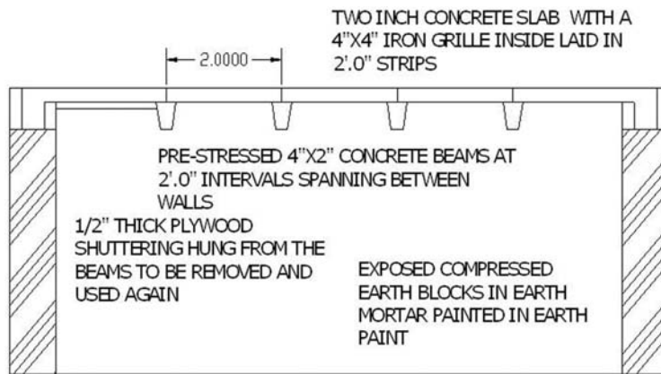
FIGURE 11. Section through the slab.
