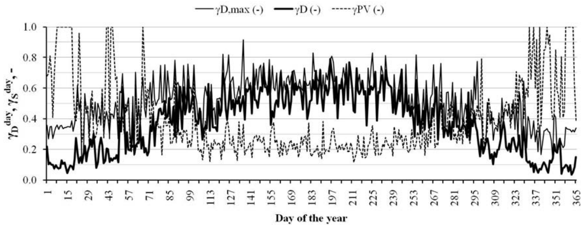
FIGURE 6. \gamma_D^{\text{day}} (bold), \gamma_{D,\text{max}}^{\text{day}} (black) and \gamma_{PV}^{\text{day}} (dashed) through the year for a modelled dwelling with space heating but without domestic hot water by means of a heat pump. A resulting \gamma^{\text{year}} of 0.29 and a value \varepsilon_{\gamma_D}^{\text{year}} of 0.46 is found.
