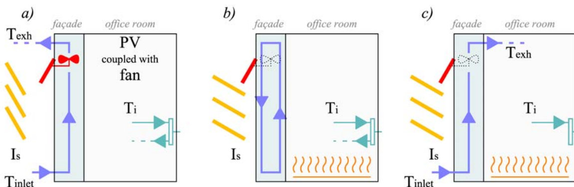
FIGURE 12. Operating strategy of the hybrid ventilated DSF—(a) summer season; (b) winter season; (c) air supply in the winter and mid-seasons.
