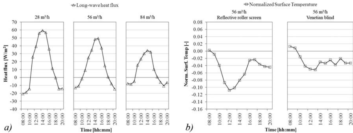
FIGURE 6. Climate façade—(a) “long wave” heat fluxes in winter conditions, configuration with venetian blind, and different air flow rates; (b) normalized surface temperature of the inner glass in summer conditions, configuration at 56 m 3 /h with different shading devices.
