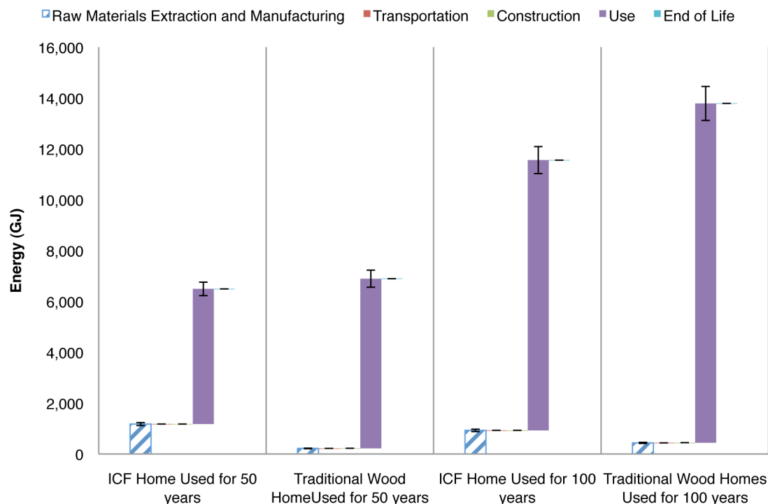
FIGURE 2. Energy consumption of ICF and wood homes for 50 and 100 year lifetimes. The positive and negative error bars are shown with an error of 5 percent. Since traditional wood homes have a lifetime of 50 years, two wood homes built for 50 years each are compared with an ICF home standing for 100 years.
