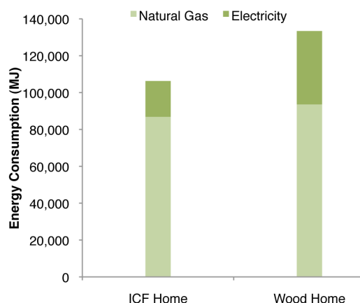
FIGURE 3. Energy consumption for wood and ICF homes for one year.
