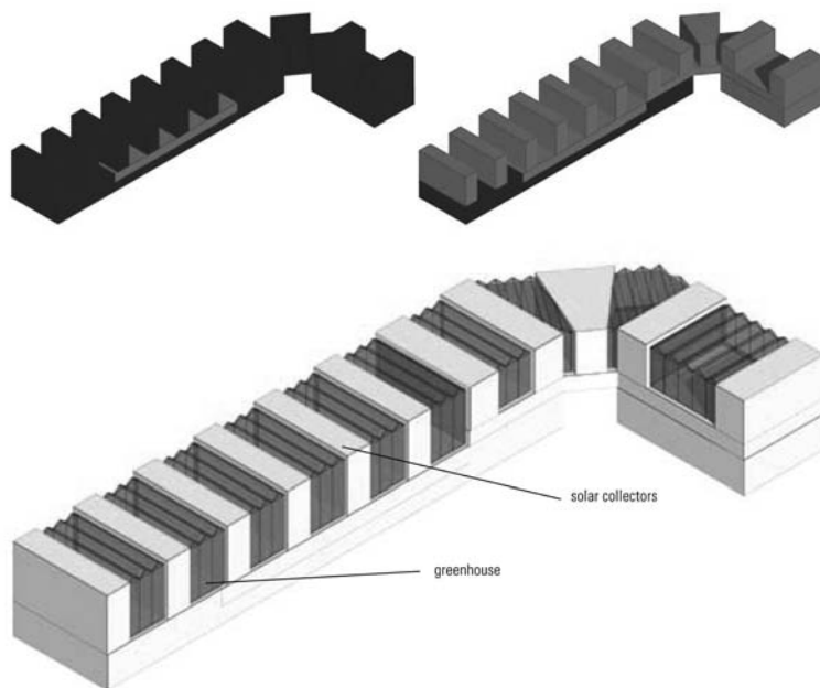
FIGURE 7. Step 01,02, summer situation energy demand total program, Heat (H), -7801 GJ, Cold (C) -13637 GJ, Electricity -6496 GJ; wintersituation in the center, energy demand total program, Heat (H), -18940 GJ, Cold (C) -7468 GJ, Electricity -6749 GJ; Right, Step 03 the resulting demand can be generated sustainably.
