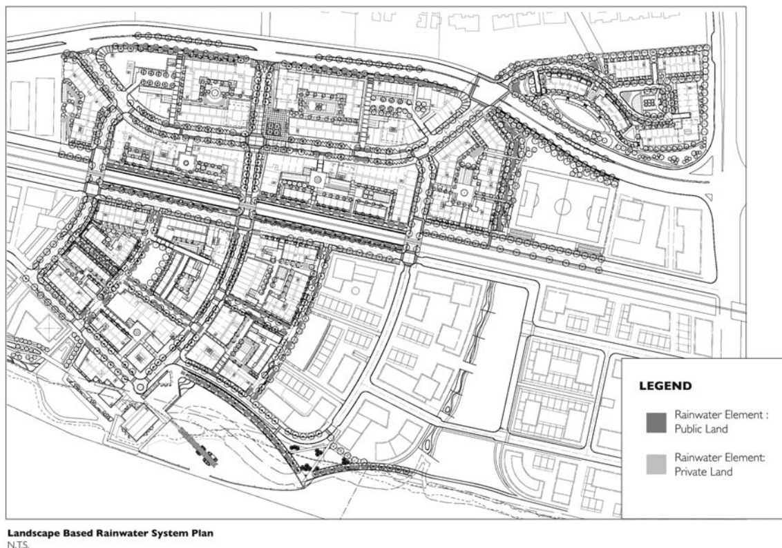
FIGURE 4. East Fraserlands Rainwater Management Plan—Phase 1, Vancouver BC.
