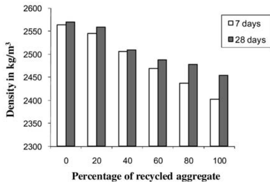
FIGURE 2. Effect of RA Content on Density.
