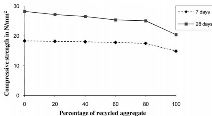
FIGURE 3. Effect of RA Content on Compressive Strength.
