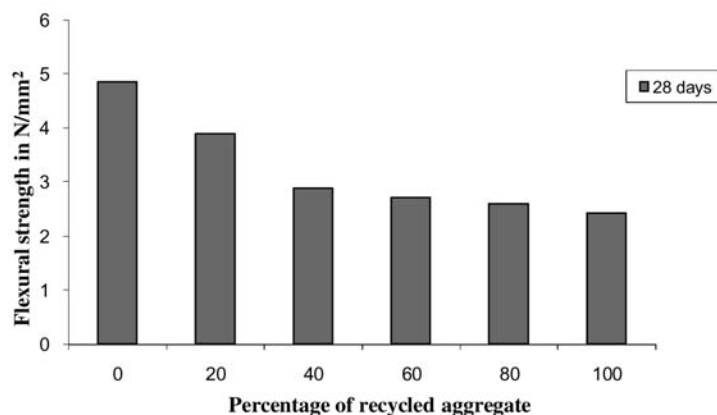
FIGURE 5. Effect of RA Content on Flexural Strength.
