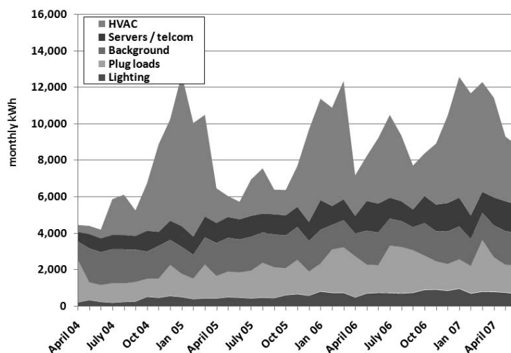
FIGURE 13. Monthly Electrical use by load type, April 2004–June 2007.
